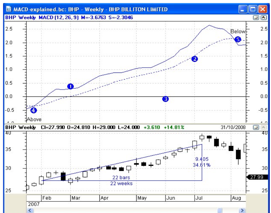
Figure 1: MACD indicator (upper pane), with BHP Weekly candles (lower pane).
